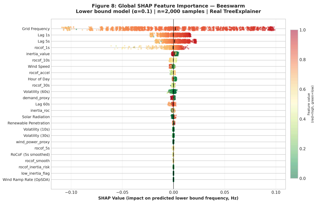
Figure 8: Global SHAP beeswarm plot detailing how feature magnitudes (e.g., extreme negative RoCoF) mathematically push the model towards an unstable frequency prediction.
